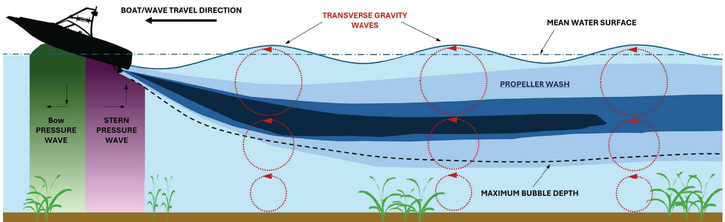
Figure 3. Illustration of the three hydrodynamic phenomena produced by a powerboat and how they interact with the water column beneath the boat.
